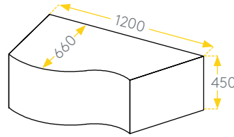
C 1200 x 660
